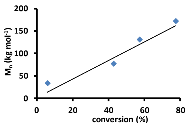
Fig. S15 Evolution of the number-average molar mass based on static light scattering detection, M_n^{LS} (◆), determined using the experimental dn/dC values, versus monomer conversion for the RAFT polymerization ( P 2 ) of DMAc at 90 °C. The straight line corresponds to the expected evolution of the theoretical number-average molar mass.
