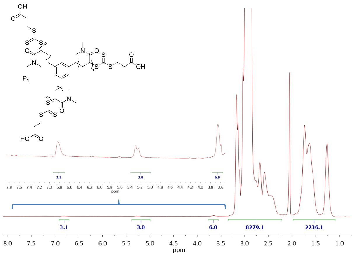
Fig. S7 ^1\text{H} NMR spectrum of the carboxylic acid-functionalized PDMAc triarm star polymer ( P_1 ) recorded in acetone- d_6 at 25°C (500 MHz).
