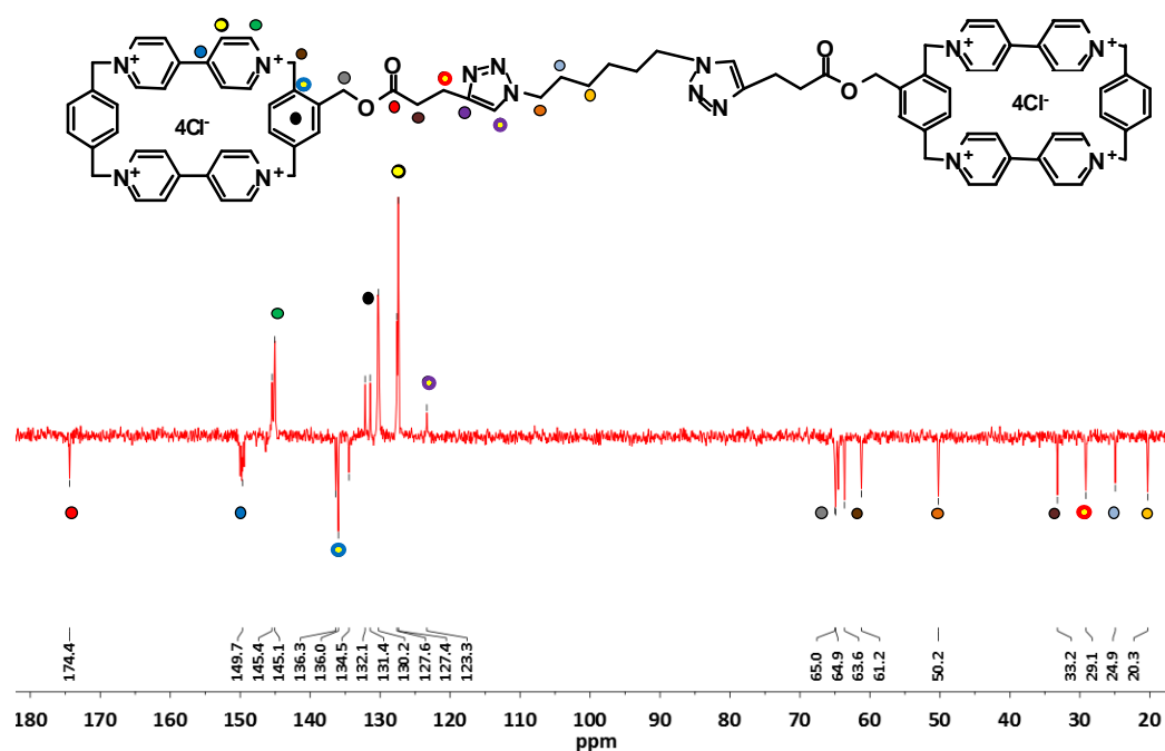
Fig. S4 ^{13}\text{C} NMR (JMOD) spectrum of the di( \text{CBPQT}^{4+} , 4\text{Cl}^- ) 6 recorded in \text{D}_2\text{O} .
