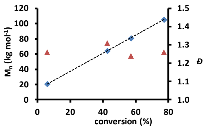
Fig. S10 Evolution of the number-average molar mass, M_n ( \blacklozenge ) and dispersity, D ( \blacktriangle ) determined by SEC in DMF (+ LiBr) using PMMA standards versus monomer conversion for the RAFT polymerization ( P_2 ) of DMAc at 90 °C.
