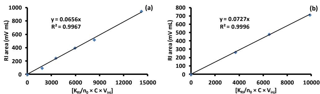
Figure S14. RI area (integrated from the RI signals with Omnisec Software) versus [K_{RI}/n_0 \times C \times V_{inj}] . (a): Results obtained from the end-chain carboxylic acid-functionalized PDMAc triarm star polymer, P 1 . (b): Results obtained from end-chain naphthalene-functionalized PDMAc triarm star polymer, P 2 .
