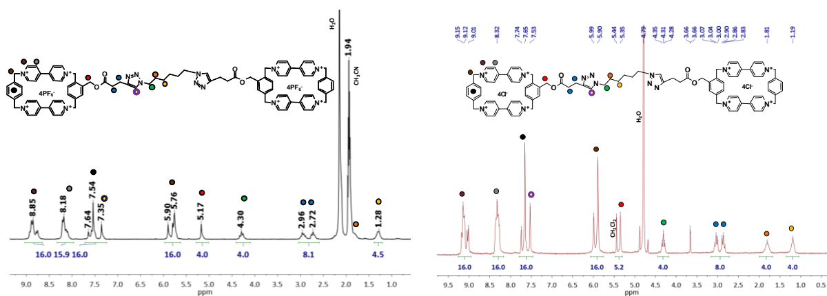
Fig. S3 ^1\text{H} NMR spectra of the di( \text{CBPQT}^{4+} , 4\text{PF}_6^- ) recorded in \text{CD}_3\text{CN} (left) and of the di( \text{CBPQT}^{4+} , 4\text{Cl}^- ) 6 recorded in \text{D}_2\text{O} (right).
