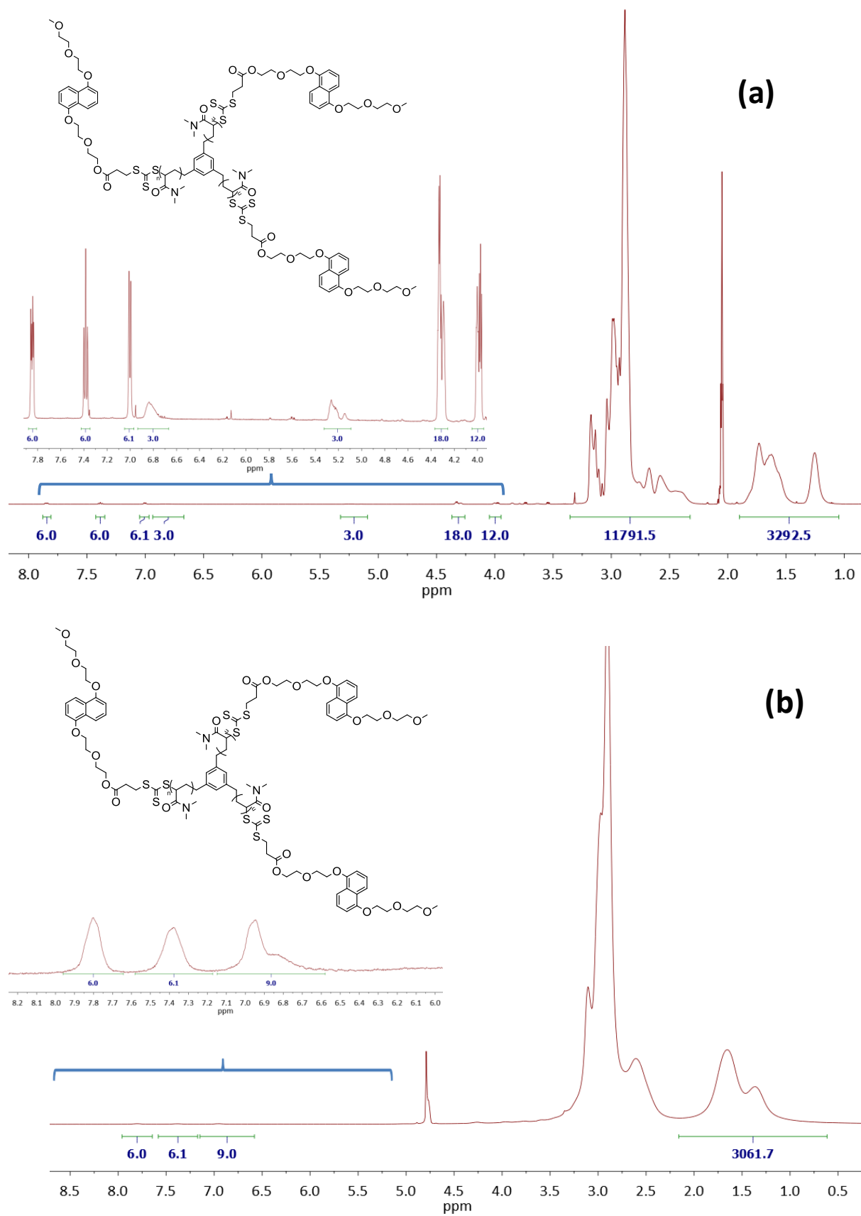
Fig. S13 ^1\text{H} NMR spectrum of the dialkyloxynaphthalene-functionalized PDMAc triarm star polymer ( \text{P}_2 ) recorded in acetone- \text{d}_6 (a) and in \text{D}_2\text{O} (b) at 25^\circ\text{C} (500 MHz).
