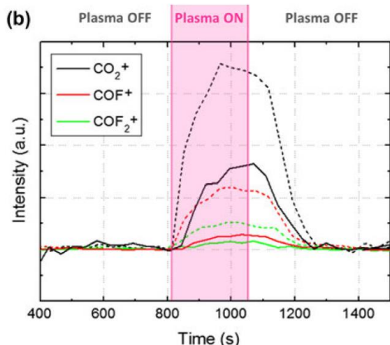
Figure 8. Intensity of the (a) CF_3^+ , C_2F_5^+ , C_3F_5^+ and C_3F_7^+ and (b) CO_2^+ , COF^+ , COF_2^+ fragments generated during the atmospheric pressure PECVD of C_6F_{14} as a function of time, in argon (full curves) and helium (dashed curves). (0.2 L/min C_6F_{14} -carrier gas, 5 L/min carrier gas total, 50 W).
