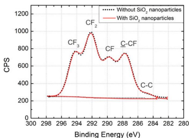
Figure 13. HR C 1s spectra of pp- C_6F_{12} films in argon with SiO_2 nanoparticles (red curve) and without SiO_2 nanoparticles (black dashed curve). (0.2 L/min C_6F_{12} -carrier gas, 5 L/min carrier gas total, 50 W).
