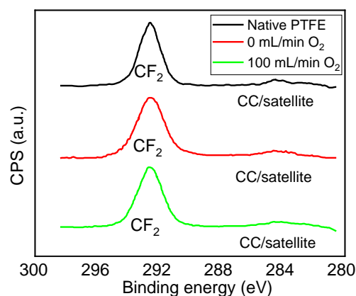
Figure 3. HR C 1s spectra of untreated PTFE and He and He- \text{O}_2 plasma-treated PTFE. ( L_s = 10 mm, v_s = 25 mm/s, g_s = 500 \mu\text{m} , N_s = 1000 , \Phi(\text{He}) = 15 L/min, \Phi(\text{O}_2) = 0 and 100 mL/min, P = 90 W).
