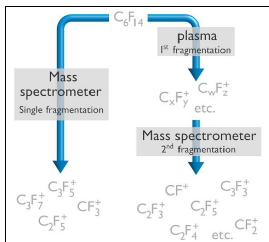
Figure 9. Scheme of the possible fragmentation of C_6F_{14} (left) in the mass spectrometer and (right) in the plasma, followed by the mass spectrometer ( C_xF_y^+ and C_wF_z^+ assuming to be CF_3^+ , C_3F_7^+ and C_3F_5^+ according to MS results).
