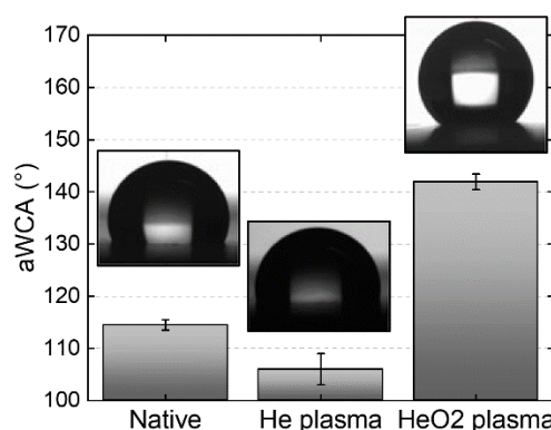
Figure 2. Advancing WCAs of untreated PTFE and He and He- \text{O}_2 plasma-treated PTFE, with the associated pictures of the static WCA. ( P = 90 W, L_s = 10 mm, v_s = 25 mm/s, g_s = 500 \mu\text{m} , N_s = 1000 , \Phi(\text{He}) = 15 L/min, \Phi(\text{O}_2) = 0 and 100 mL/min).
