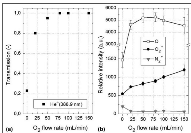
Figure 6. (a) Transmission rate of He 2^3\text{S} at 388.9 nm and (b) optical emission intensity of O (844.6 nm), \text{O}_2^+ (525 nm) and \text{N}_2^+ (391 nm) in the He- \text{O}_2 post-discharge ( g_s = 1 mm, \Phi(\text{He}) = 15 L/min, P = 120 W).
