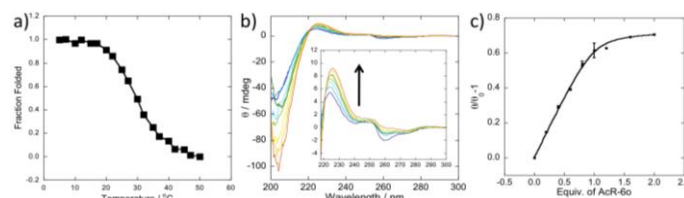
Figure 2. Thermal denaturation of R2-6/AcR-6o 1:1 mixture (a) and titration experiment monitored by circular dichroism (b) and (c). The titration was performed at 20°C at 5 \mu M in phosphate buffer (10 mM, pH = 7.2) and (c) shows the titration curve monitored at 225 nm. The inset of (b) shows a zoom of the monitored band at 225 nm. Error bars represent the standard deviation.
