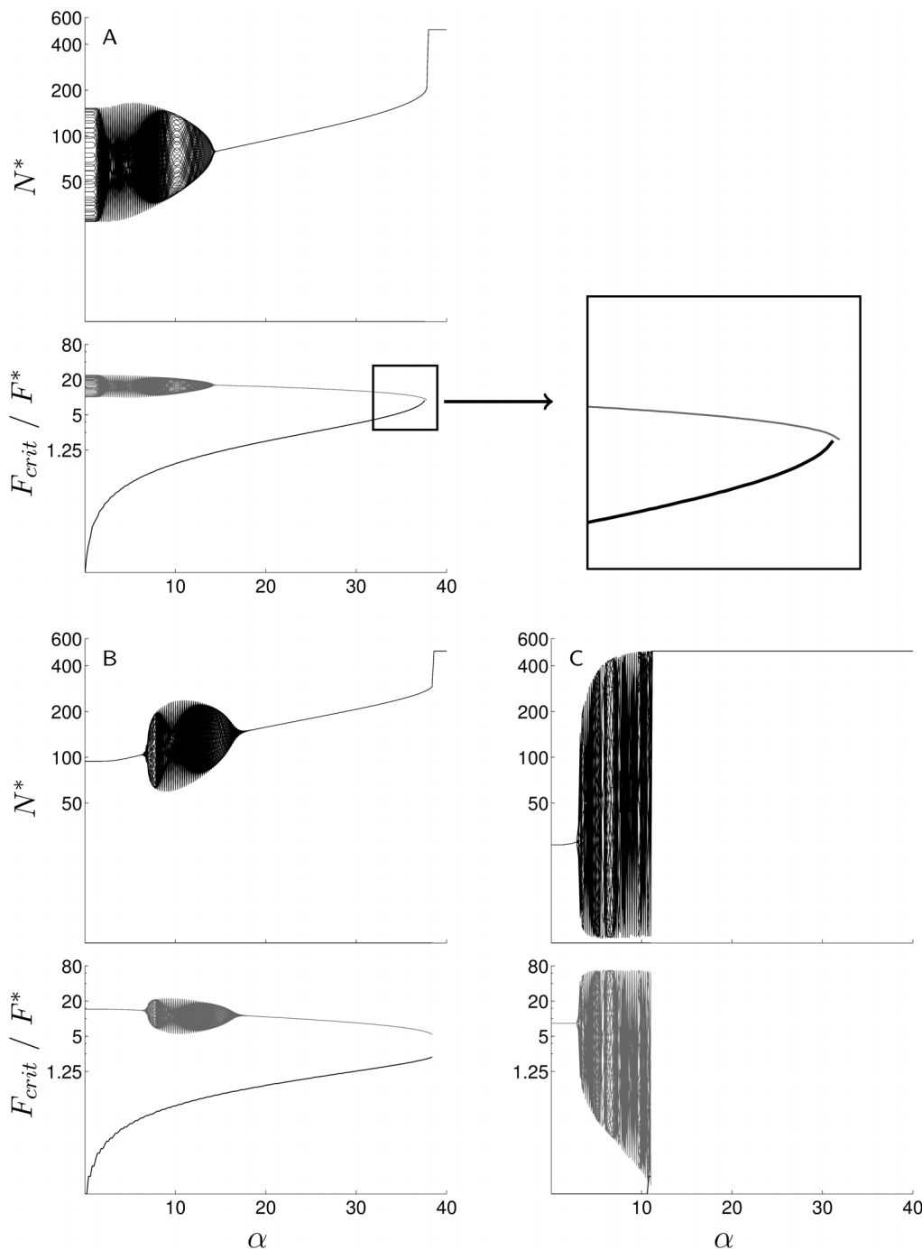
Figure 4. Bifurcation diagrams for hosts (black) and parasitoids (gray) populations, as a function of the intensity of a mate-finding Allee effects ( \alpha ). Population characteristics: a) k = 10 , b = 1.5 , a = 0.14 , \lambda = 12.2 ; b) k = 10 , b = 0.8 , a = 0.058 , \lambda = 4 ; c) k = 0.8 , b = 1.5 , a = 0.25 , \lambda = 2.85 . The black curve on parasitoid graphics represents F_{crit} . doi:10.1371/journal.pone.0076768.g004
