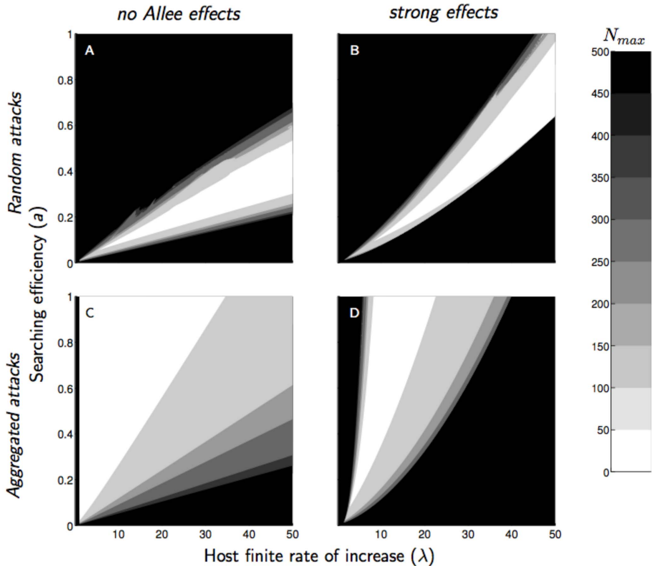
Figure 6. Residual host abundance after parasitism ( N_{\max} ) without ( \alpha=0 ) and with ( \alpha=20 ) a strong mate-finding Allee effect and either a random ( \kappa=10 ) or aggregated ( \kappa=0.8 ) distribution of attacks, as a function of parasitoid searching efficiency ( a ) and host finite rate of increase ( \lambda ). Intraspecific competition in the host population was assumed medium ( b=1.5 ) doi:10.1371/journal.pone.0076768.g006
