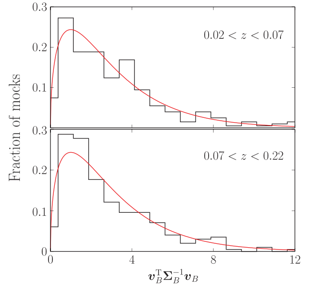
Figure 2. Distribution of the quadratic form \mathbf{v}_B^T \Sigma_B^{-1} \mathbf{v}_B derived from the SDSS mock catalogues, assuming the Schechter model of the LF: the histograms represent the observed (normalized) distribution and solid lines correspond to the \chi^2 -distribution with k = 3 degrees of freedom.
