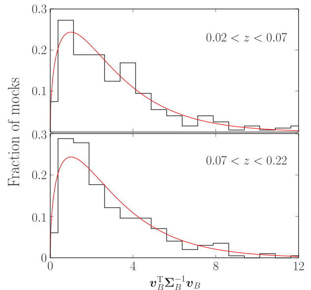
Figure 2. Distribution of the quadratic form \mathbf{v}_B^T \Sigma_B^{-1} \mathbf{v}_B derived from the SDSS mock catalogues, assuming the Schechter model of the LF: the histograms represent the observed (normalized) distribution and solid lines correspond to the \chi^2 -distribution with k = 3 degrees of freedom.
