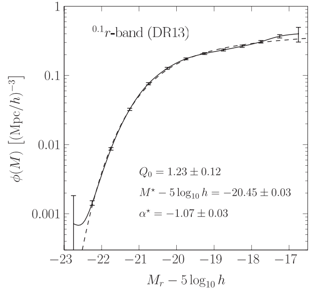
Figure 1. The ^{0.1}r -band LF of the luminosityA sample from the SDSS DR13: illustrated are the maximum-likelihood result adopting the spline-based estimator with \Delta M = 0.5 (solid line), and a fit based on the Schechter model (dashed line). Error bars correspond to marginalized 99.7 per cent confidence limits of individual spline points.
