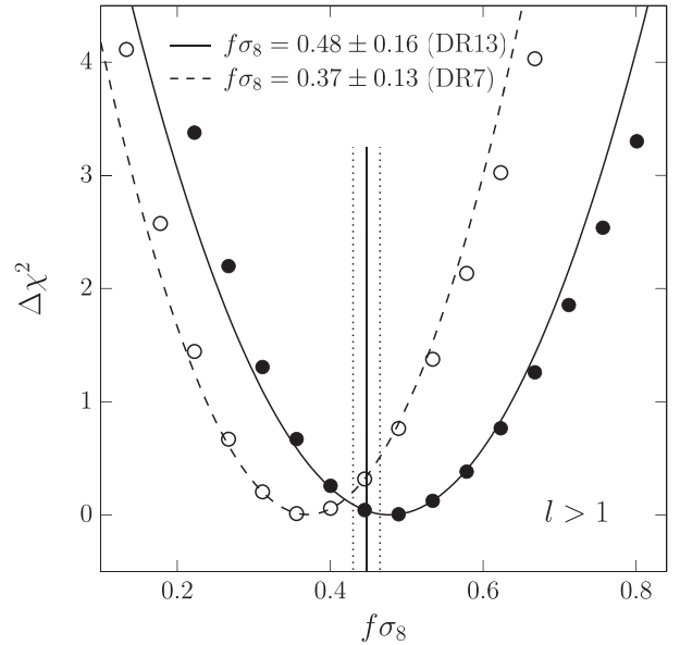
Figure 3. Estimated \Delta\chi^2 (and its quadratic approximation) as a function of f\sigma_8 for linear velocity models with l > 1 . Presented are results based on galaxies from SDSS DR13 (filled circles) and DR7 (open circles). The estimates assume the power spectrum amplitude of L^* -galaxies given by Tegmark et al. (2004). Vertical lines indicate the result inferred from Planck data (TT + lowP + lensing; Planck Collaboration XIII 2016) and its 95 per cent confidence limits.
