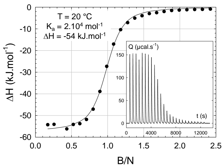
Figure 3. Isothermal calorimetric titration ( T=20\text{ }^{\circ}\text{C} ) of a P(DMA-N1) aqueous solution ( [\text{N}]=0.4\text{ mM} ) with B ( [\text{B}]=30\text{ mM} ).
