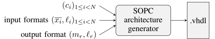
Fig. 6. Interface to a sum-of-product-by-constant generator
