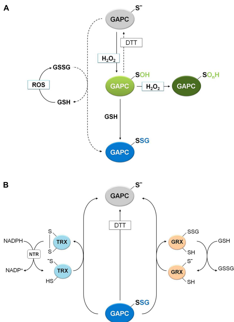
FIGURE 5 | Molecular mechanisms of plant GAPC glutathionylation and deglutathionylation. (A) Oxidation and glutathionylation of plant GAPC. Plant GAPC can undergo primary oxidation to sulfenic acid (GAPC-SOH) in the presence of H_2O_2 that can subsequently react with GSH leading to the glutathionylated form (GAPC-SSG) and protecting the enzyme from irreversible oxidation (GAPC-SO n H). In principle, GAPC glutathionylation may also be performed by GSSG with release of GSH, but this reaction does not occur under physiological GSH/GSSG ratios (dashed arrow). GSSG can be formed by the reaction of GSH with
