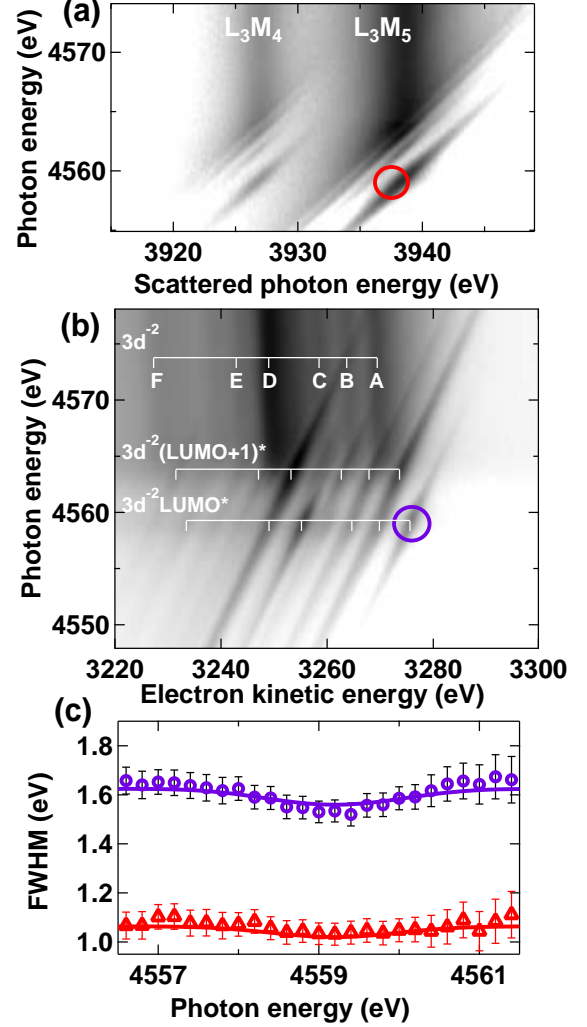
FIG. 1: (a) RIXS L_3M_{4,5} and (b) Auger L_3M_{4,5}M_{4,5} spectra recorded in CH_3I near the I L_3 edge. A detailed assignment of the labeled Auger lines is presented in the Supplemental Material. (c) FWHM of RIXS emission line (triangles) and Auger line (circles) selected in (a) and (b), respectively, as a function of photon energy around the LUMO resonance. Error bars are obtained from the fits of the experimental spectra. Solid lines show simulations based on Eqs.2 and 3.
